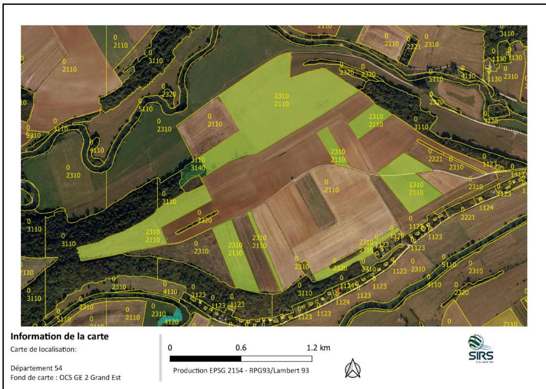
Figure 16 : Image 2010 : Prairies
