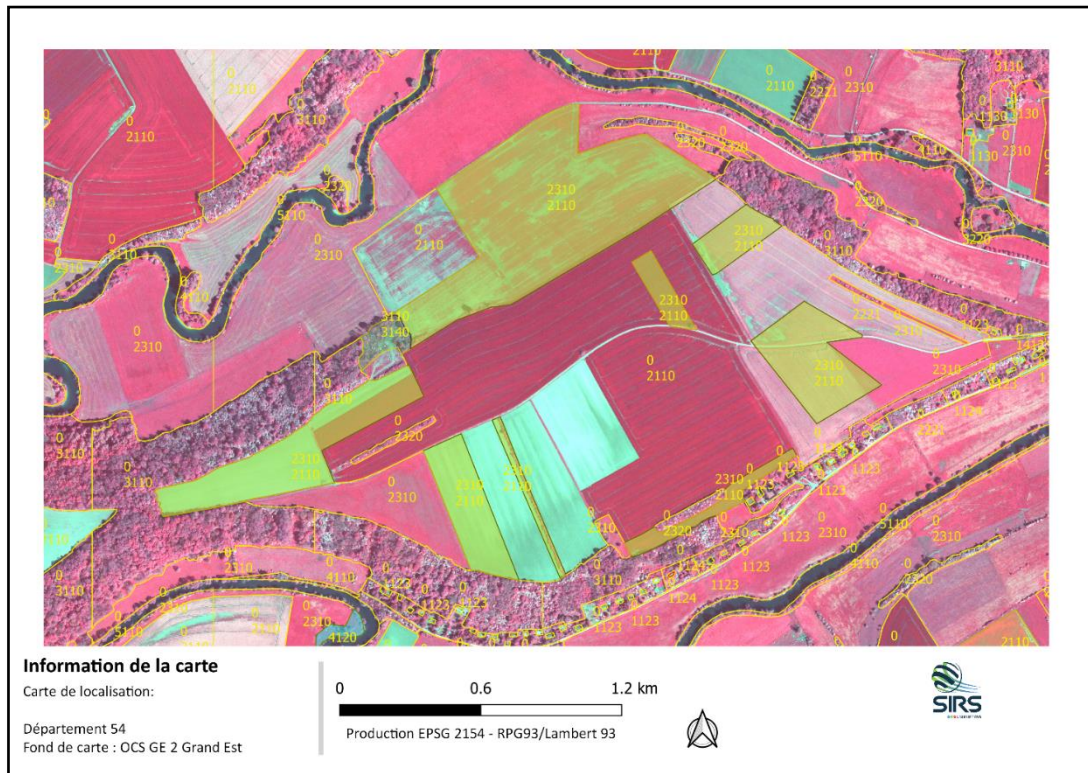
Figure 15 : Image 2019 : cultures
