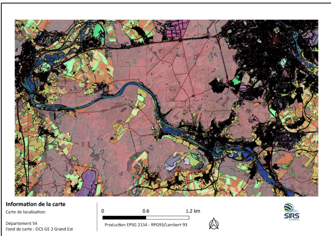
Figure 7 : Couvert forestier
